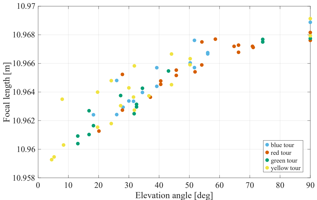
Figure 9: Elevation-dependent focal lengths
