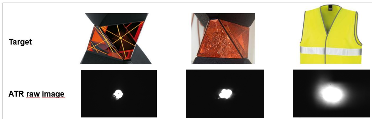
Figure 3 Environmental effect on prism recognition
