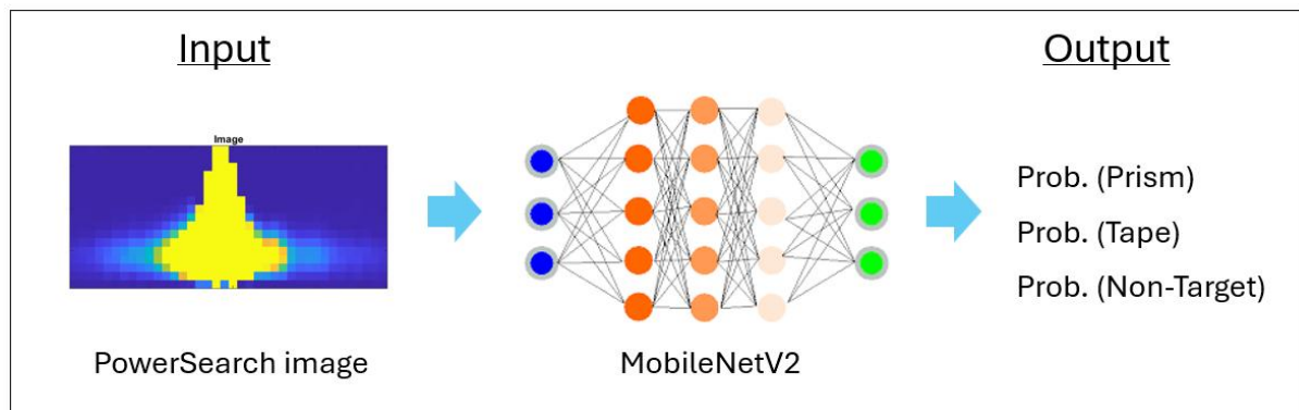
Figure 2 Visualisation of the MobileNetV2 algorithm
