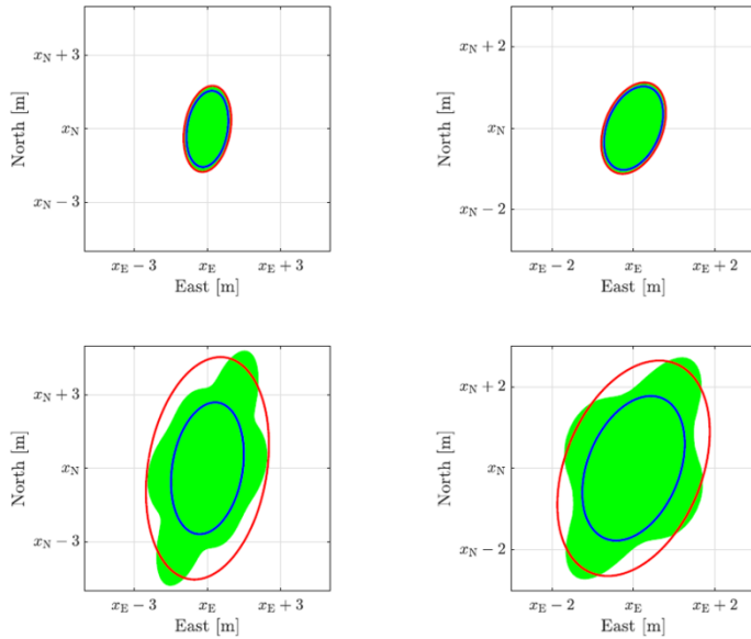
Fig 3: Illustration of confidence regions for the two skyplots of Figure 2, with \alpha = 0.1 (top) and \alpha = 0.001 (bottom): C_\alpha^{DIA} is indicated by the green area and C_\alpha by the blue ellipse.
