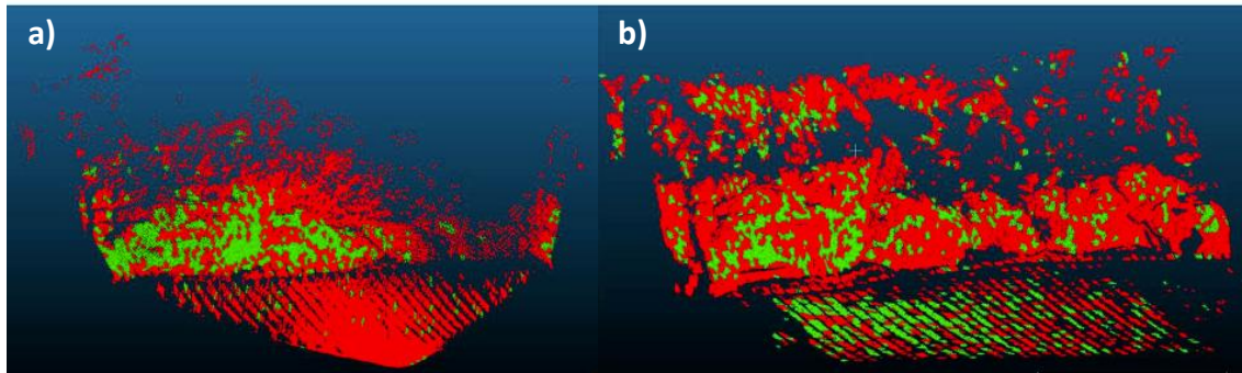
Figure 2: Spatial distribution of stable (green) and unstable (red) regions identified by Piecewise-ICP registration method. (a) Results for the Livox. (b) Results for the RIEGL.
