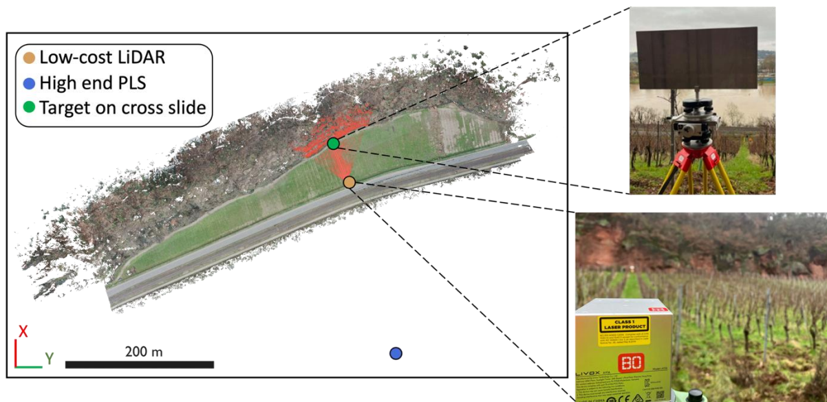
Figure 1: Sensor configuration at the Trierer Augenscheiner showing the high-end z zPLS installation, the low-cost LiDAR sensor, and the planar target used for the controlled displacement experiment.
