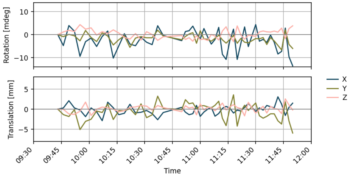
Figure 4: Estimated transformation parameters obtained from the registration of consecutive point clouds for the Livox sensor. Rotational parameters are shown in the upper panel and translational parameters in the lower panel.
