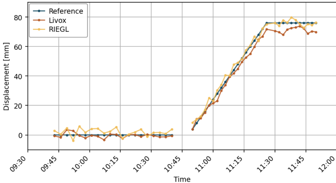
Figure 5: Time series of the plane-based displacement measure c during the controlled displacement experiment. The data gap between 10:40 and 10:50 represents a scheduled pause separating the initial static phase from the subsequent displacement phase, while the sensor systems remained powered on.
