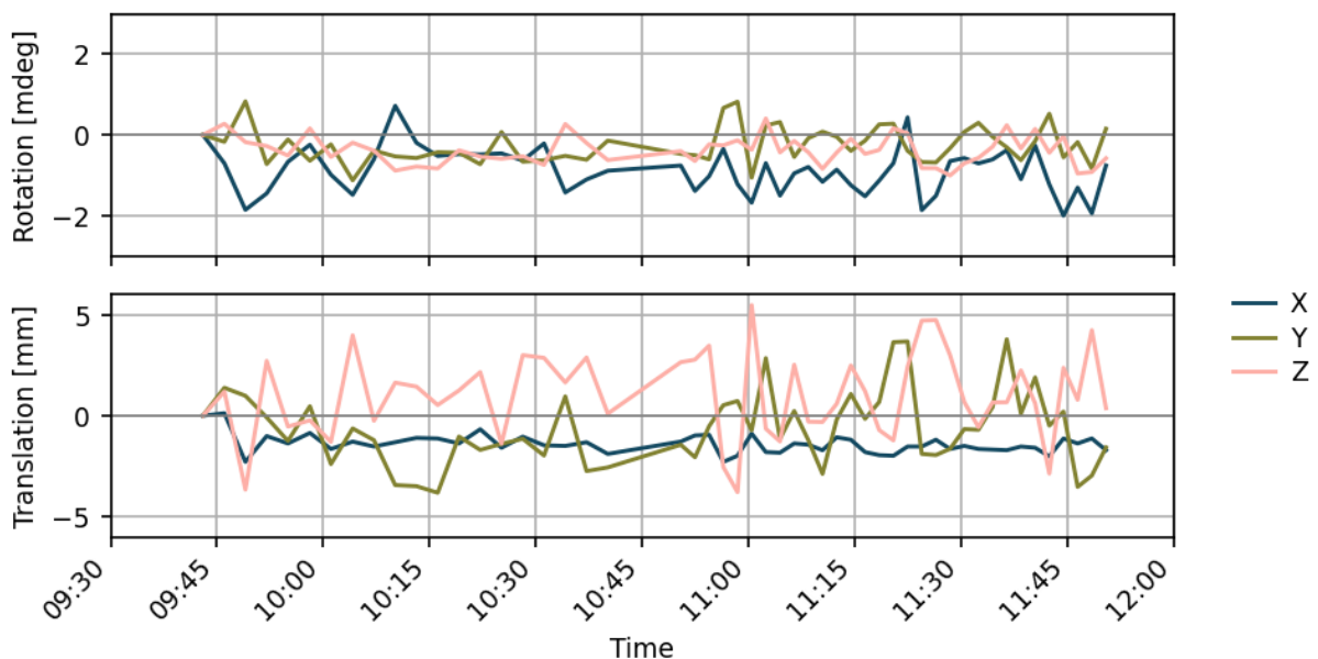
Figure 3: Estimated transformation parameters obtained from the registration of consecutive point clouds for the RIEGL system. Rotational parameters are shown in the upper panel and translational parameters in the lower panel.
