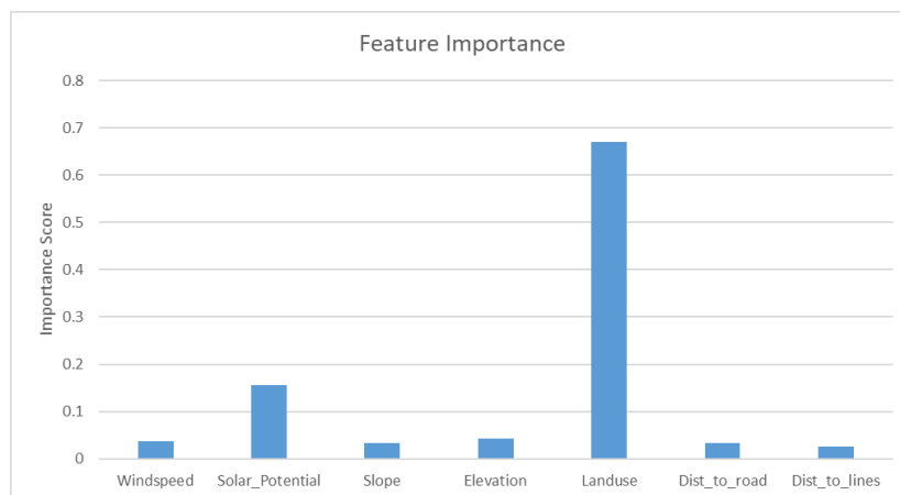
Figure 6: Feature Importance
