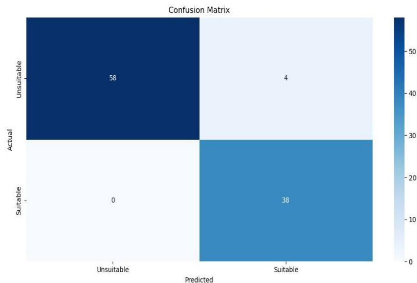
Figure 5: Confusion matrix
