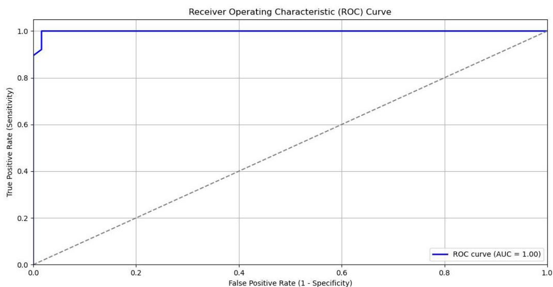
Figure 7: Model Validation
