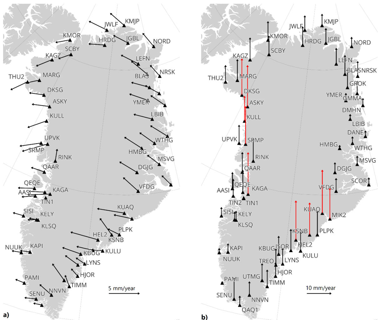
Figure 2. Velocities of GNET stations based on data from Berg et al. (2024). a) Horizontal velocity after correcting for plate motion. b) Vertical velocity. Red arrows indicate velocity higher than 10 mm/year.
