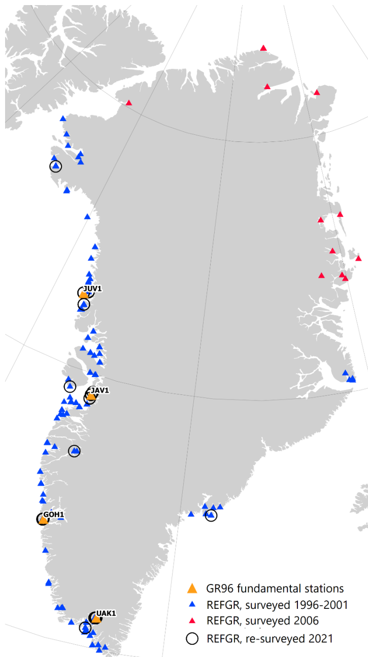
Figure 1. REFGR benchmarks established between 1996 and 2006.
