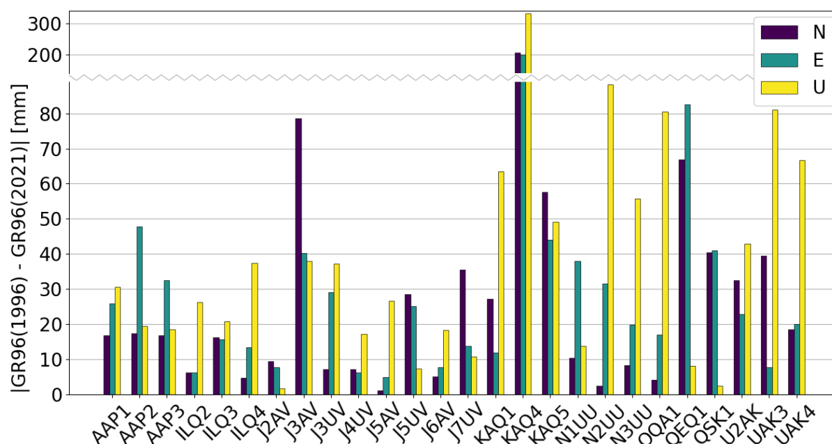
Figure 3. Validation of transformed GR96(2021) coordinates compared to GR96(1996). The figure shows the absolute differences in coordinates. Note the broken y-axis that shows the outlier at KAQA4.
