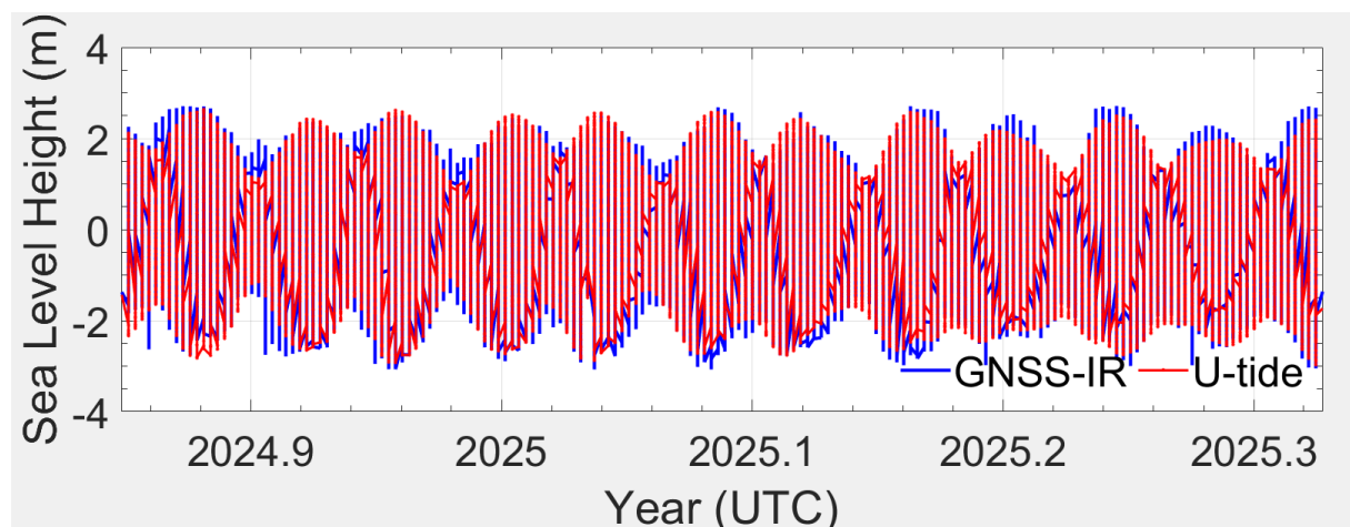
Figure 2: UTide Analysis
