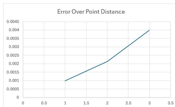
Figure 5 Error Over Point Distance GNSS
