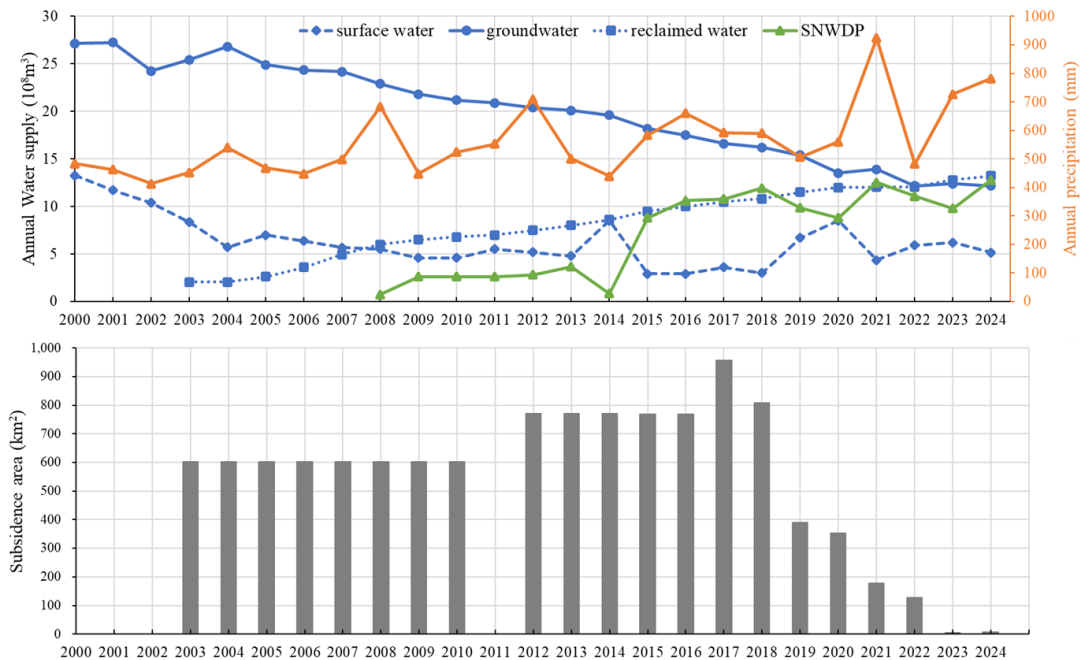
Fig. 3. Annual precipitation and water supply composition in Beijing (2000–2024) (upper panel); annual total area of severe and moderately severe subsidence (2003–2024) (lower panel).
