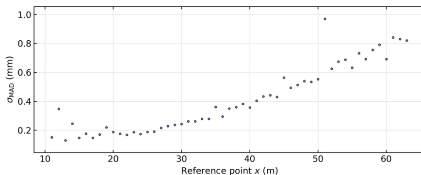
Figure 5: \sigma_{\text{MAD}} values of the detrended \Delta Z time series as a function of the reference position along the girder.
