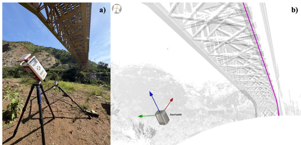
Figure 2: Field setup at the Puente Las Cucharas bridge. (a) Final scan position with the terrestrial laser scanner mounted in the 45° Tilt Mount for VZ-600i. (b) Screenshot from RiSCAN PRO showing the registered 360° overview scan (dark colour) and the corresponding high-rate line scan (magenta) aligned with the girder on the northern side of the bridge.
