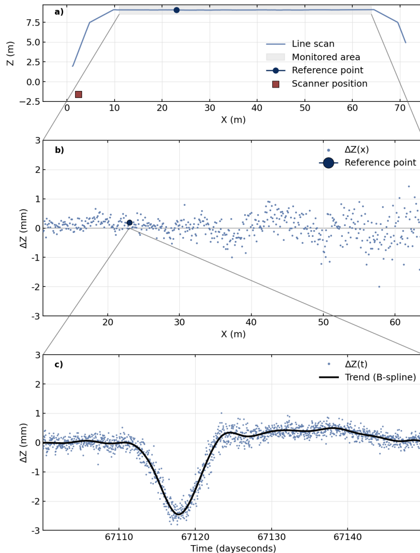
Figure 3: Line scan results for a representative train passage. (a) Longitudinal profile of the monitored girder in the LLCS ( x = 11\text{--}64 m) with scanner position. (b) Spatial \Delta Z profile at 18:38:02 UTC, including the reference position. (c) \Delta Z time series at the reference position ( x = 23 m) with B-spline trend.
