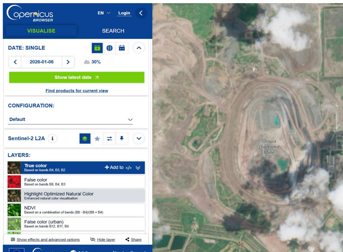
Figure 1: Location of major mining areas in Botswana (Source: Copernicus Sentinel-2, European Union and Google Earth)
