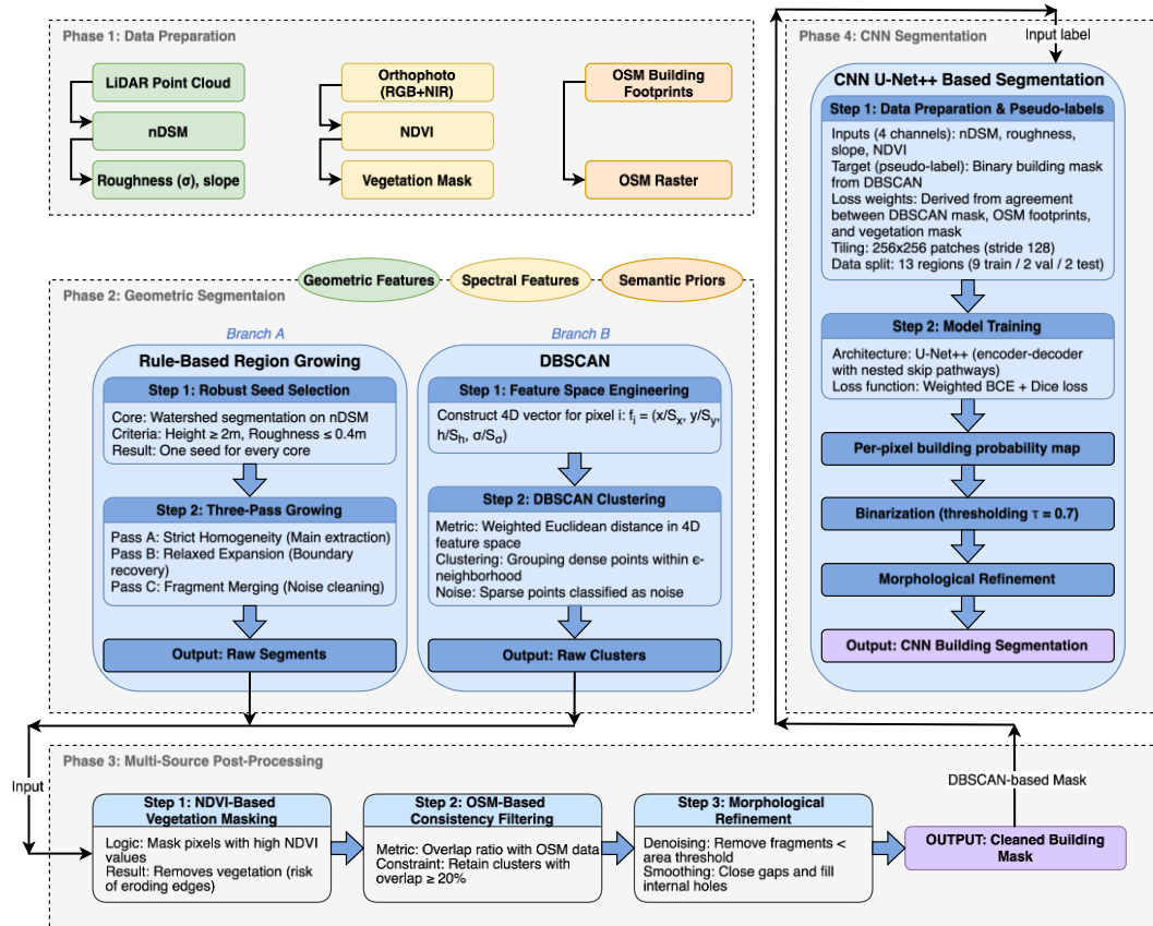
Figure 6 – DEM semantic segmentation framework: nDSM-derived geometric features, spectral vegetation information, and OSM building footprints are integrated as geometric, spectral, and semantic priors, respectively. The region growing approach identifies building seeds from the nDSM using height and roughness constraints and expands regions in multiple passes to recover building boundaries. The DBSCAN approach clusters pixels into building candidates in a normalized four-dimensional feature space (spatial coordinates, height, and local roughness) using density-based clustering. The geometric segmentation results are refined through post-processing to produce cleaned building masks, which are subsequently used as pseudo-labels for training the U-Net++ model.
