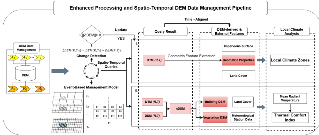
Figure 2 – Details of enhanced processing and spatio-temporal DEM data management pipeline. Our output can e.g. be used to support urban climate analysis such as change detection in LCZ and modeling of thermal comfort.
