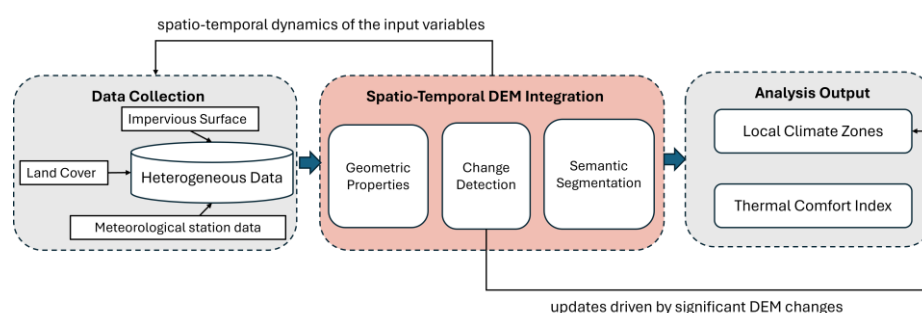
Figure 1 – The here introduced spatio-temporal DEM integration is designed to act as a central part of an enhanced urban climate analysis workflow.
