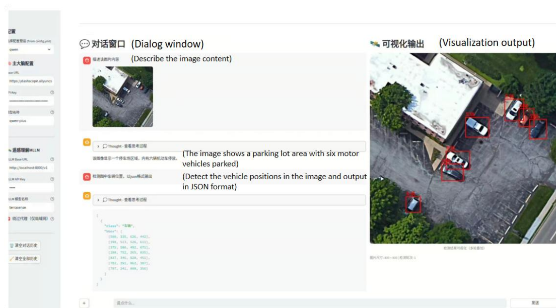
Figure 1. The interactive of user interface of the TerraSense Agent.
