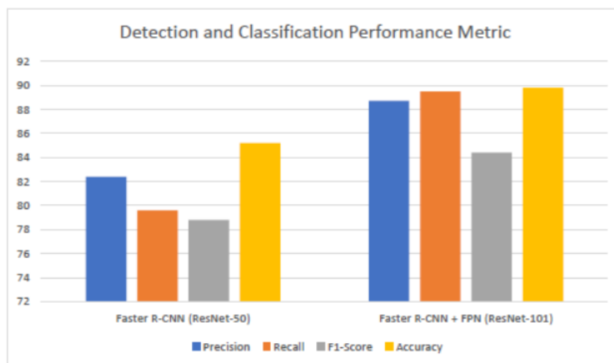
Figure 5: Detection and Classification Performance Metric
